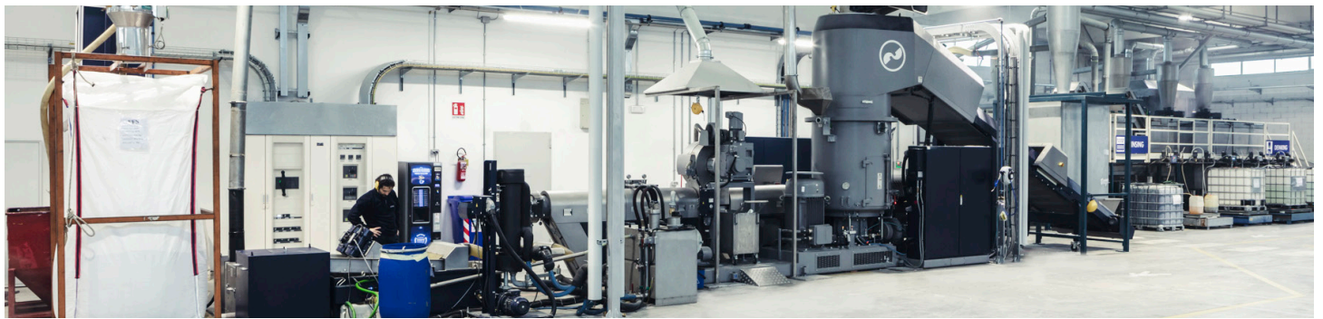
The recycling line at the Santa-Margherita plant, Italy where bags are sorted, washed, de-inked, and re-pelletized into a premium recycled product.
